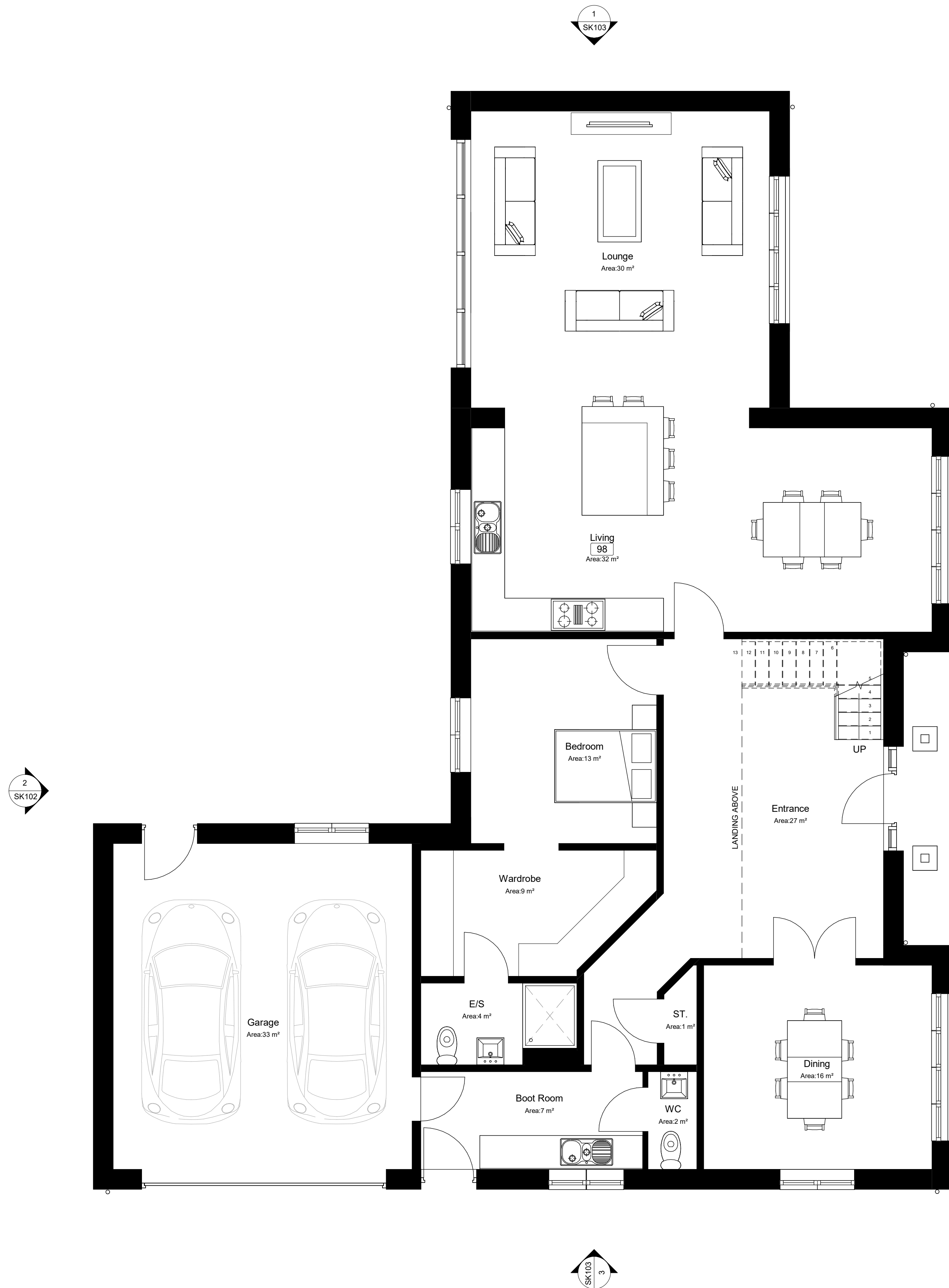
1. Proposed Ground Floor 1 : 50@A1
