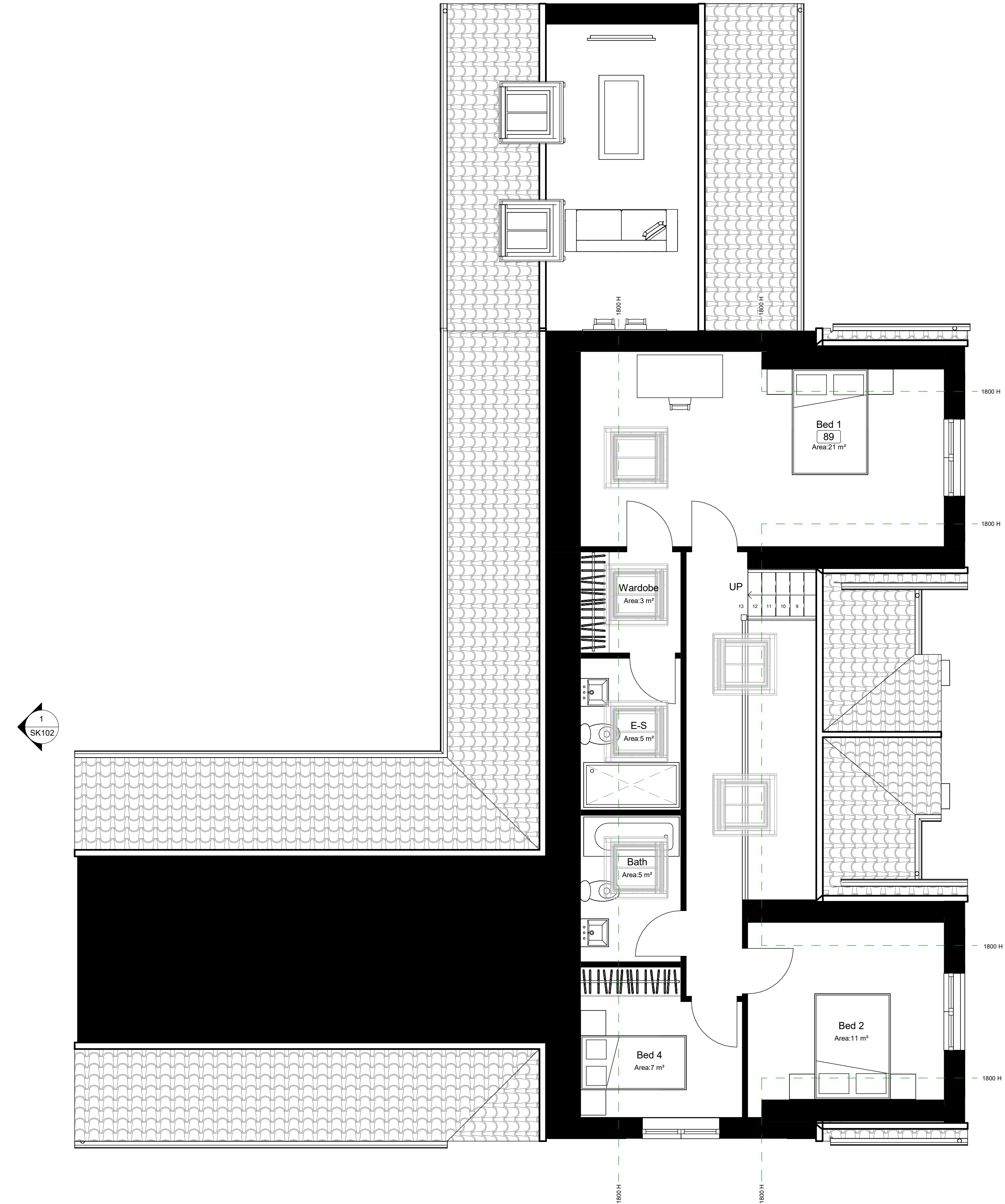
2. Proposed First Floor 1 : 50@A1
